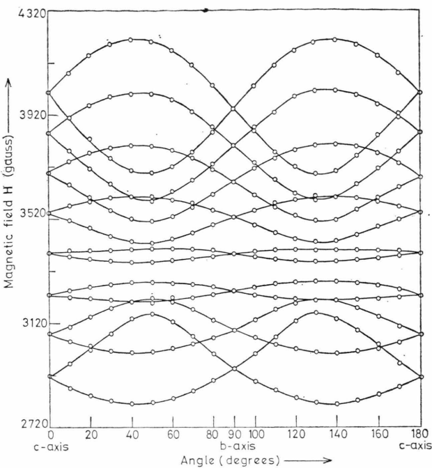
Fig. 1. Angular variation of the magnetic field at resonance in the bc plane for \text{VO}^{2+} in \text{ZnCs}_2(\text{SO}_4)_2 \cdot 6\text{H}_2\text{O} . The solid lines are smooth curves that connect data points from the same transition. This figure is for the more populous of the two \text{VO}^{2+} orientations in the Tutton salt.
